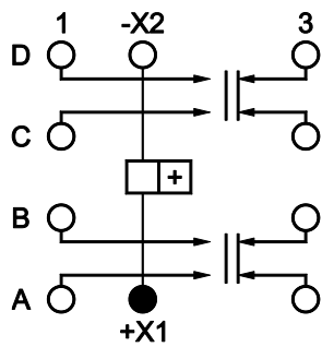
BOTTOM VIEW, DE-ENERGIZED COIL VUE DE DESSOUS, BOBINE NON ALIMENTEE
