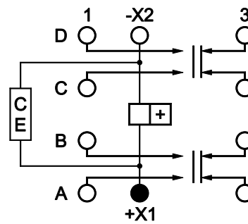
CE: SUPPRESSOR DEVICE CE: CIRCUIT ECRETEUR BOBINE
